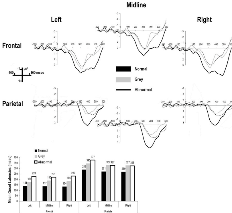
Figure 4. Top: This figure displays the waveforms resulting from go minus no-go ERPs subtraction ( n = 18 ), computed for each colour condition separately and for each scalp electrode site. A 20 Hz low-pass was used for the display. Bottom: Histograms displaying the onset latencies of significant go–no-go statistical differences for colour conditions separately.
